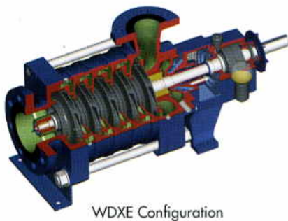
WDXE Configuration
