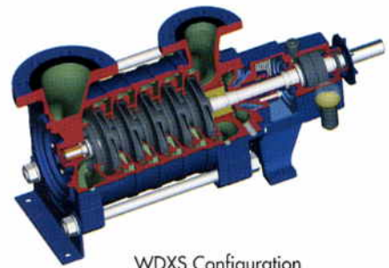
WDXS Configuration
